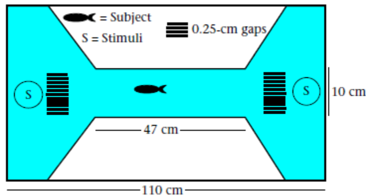
Figure 1. Diagrammatic representation of the experimental apparatus showing the runway with a conical end opening out to the slatted barrier around which the fish must detour while inspecting the stimulus partially obscured behind it.
